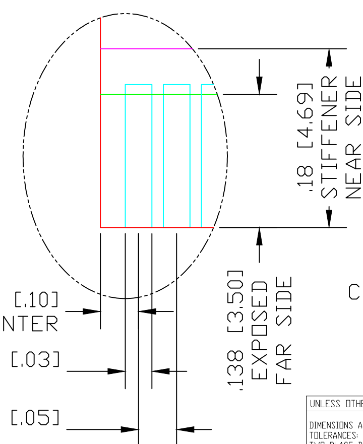
DETAIL A SCALE 10:1
